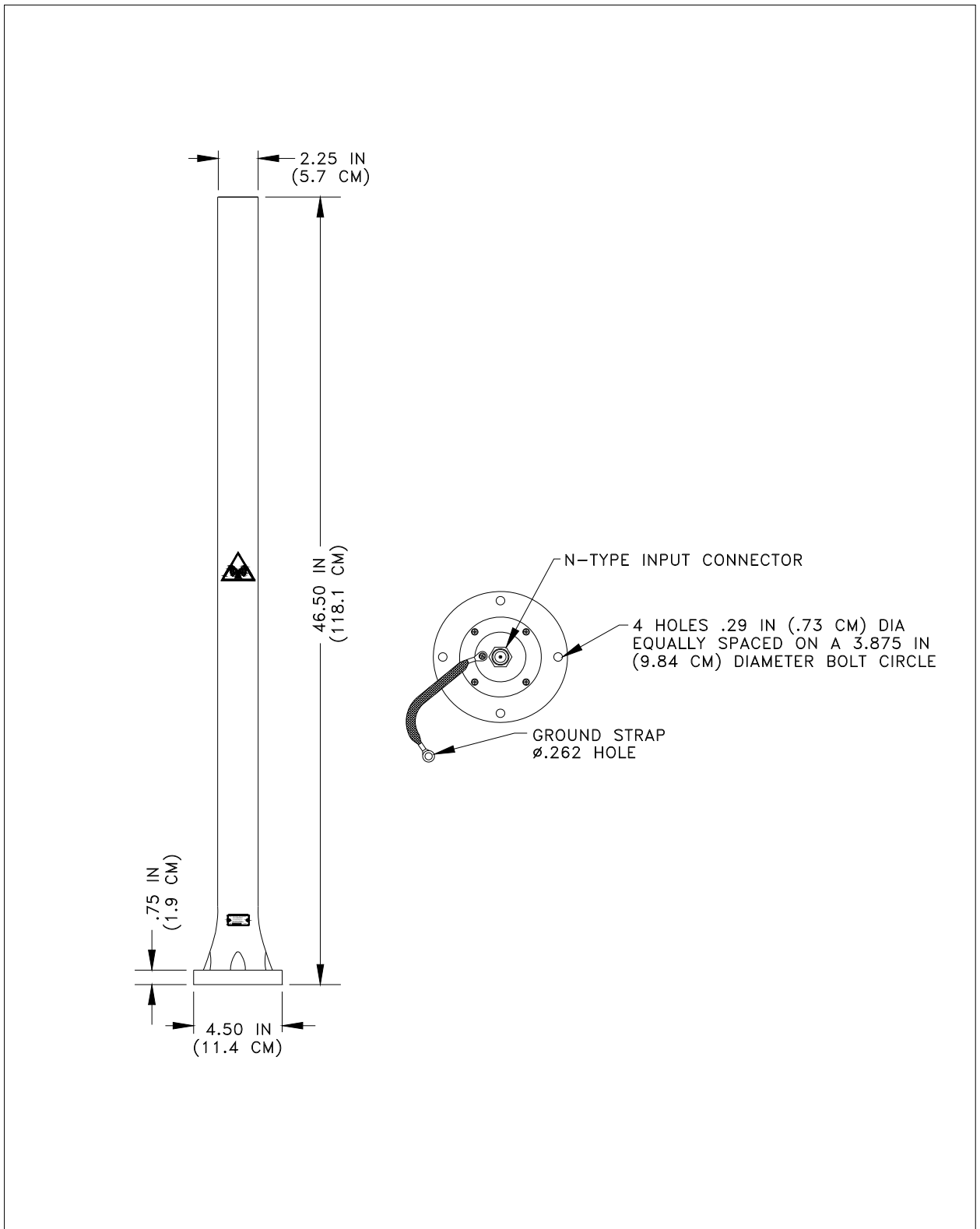
Figure 4.1 - Dipole VHF Antenna AS-2809/SRC
